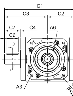
R 軸 Shaft Direction
