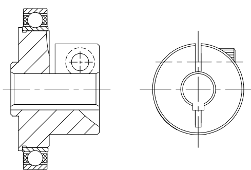
Collet + Keyway
